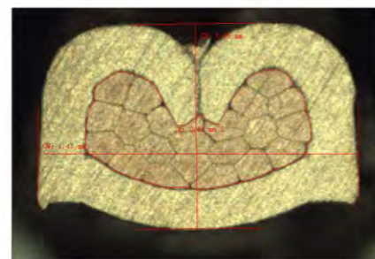
Compound type terminal
