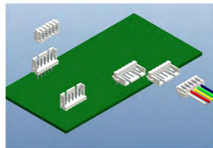
2.0 Pitch IDC
