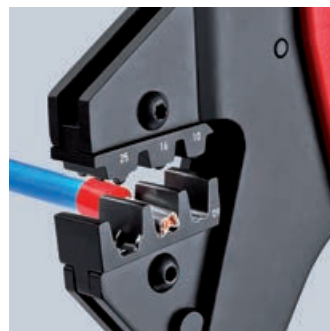
97 43 200 with crimping dies 97 49 09 for wire ferrules
