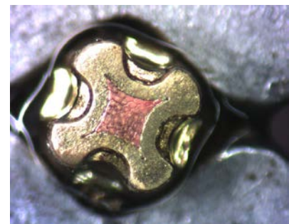
4/8-indent crimp
